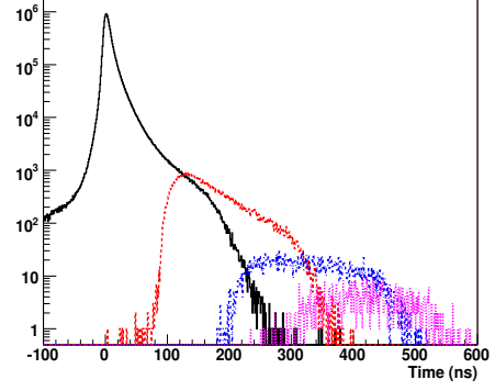
Figure 2. Time distributions of 1st (99.38 %), 2nd (0.58 %), 3rd (0.03 %) and 4th hits on the same pad.
