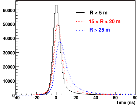
Figure 1. Shower time profile for different intervals of hit distance R from the reconstructed core.
