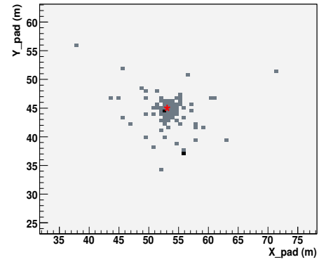
Figure 6. Space pattern (at pad level) of a very localized shower event. The spot dimensions are few meters.
