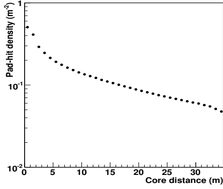
Figure 3. Lateral density profile of pad-hits with respect to the reconstructed core position.
