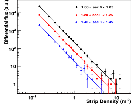
Figure 4. Differential strip density spectrum measured for different intervals of the zenith angle.
