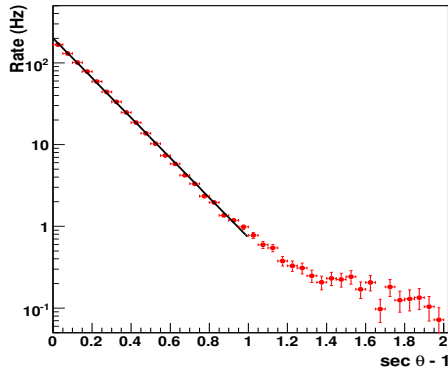
Figure 5. Zenith angle distribution of detected showers. The slope parameter for \sec\theta < 2 is \alpha = 5.62 \pm 0.11 .
