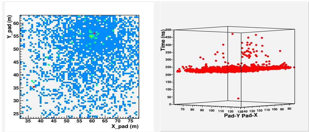
Figure 7. Display of a very large shower imaged by ARGO-YBJ. The left picture shows the space pattern (at pad level), with the reconstructed core represented by a star. In the right plot, the space-time profile of the same event can be observed.
