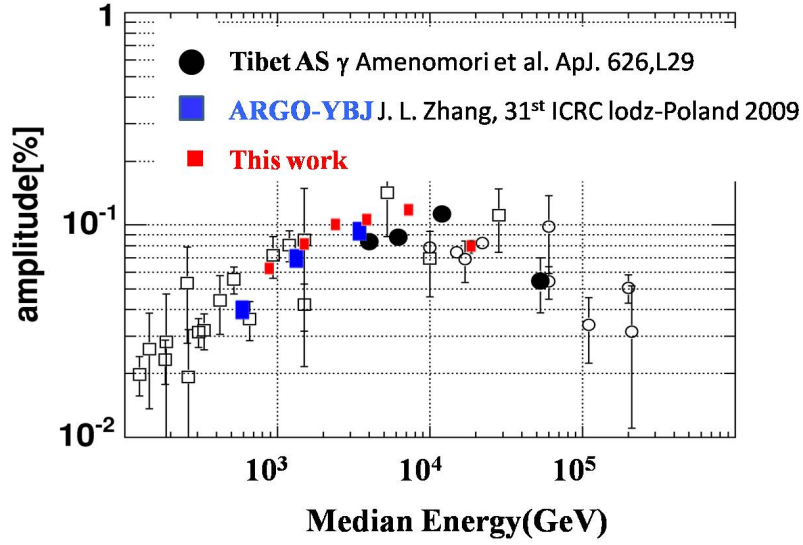
Figure 4: The amplitude of CR anisotropy intensity variation as a function of CR's median energies(in the unit of: GeV). Compared with the result other experiments especially from Tibet AS \gamma experiment[12] and presented by ARGO-YBJ last ICRC[6].
